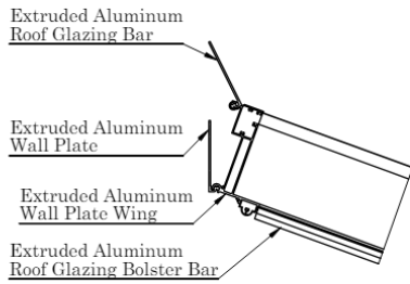
Wall Plate & Roof Bar Section
