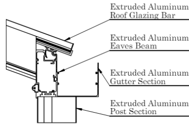
Eaves Beam Roof Bar & Post Section
